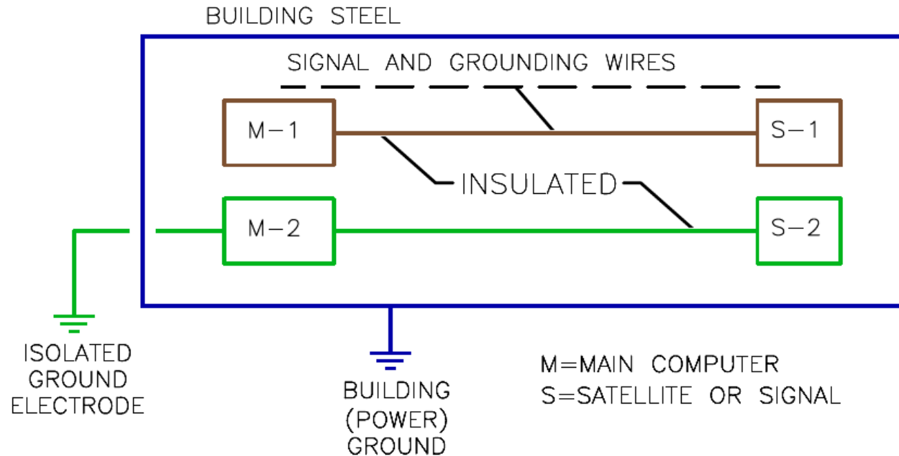
Figure 5-4—Isolated grounding of computers
